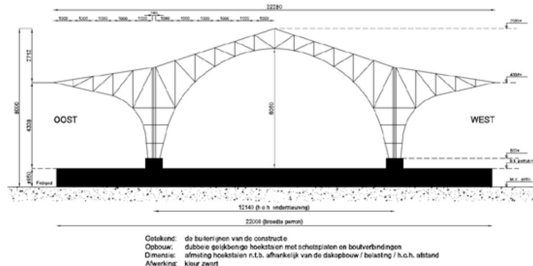
SCHEMA SPANT PERRON GRENS BAARLE-NASSAU / RAVELS
